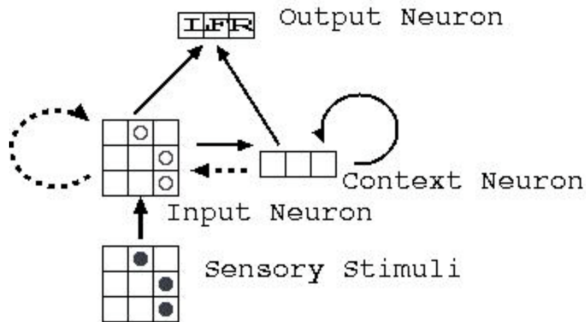
Figure 2. The design of the neural network that controlled the artificial creature's "behavior" (Adapted from Morimoto & Ikegami 2004)
